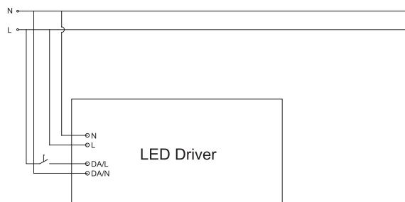
Push Dimming Connection
