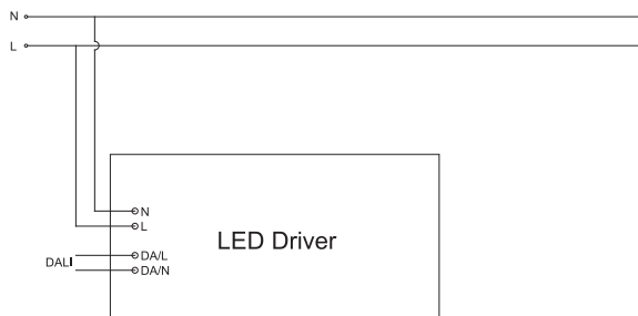
Dali Dimming Connection
